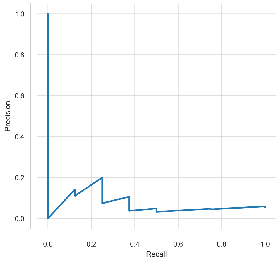
Precision-Recall Curve - SVC
